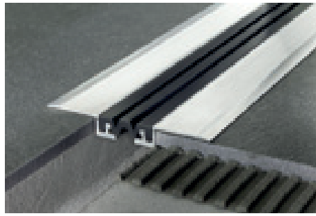
GJF/40 natural aluminium + EPDM black RAL 9005
